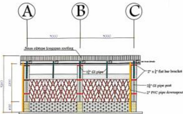
FRONT ELEVATION
