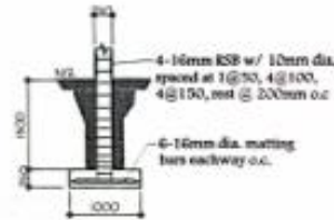
COLUMN-FOOTING DETAILS SCALE 1:500
