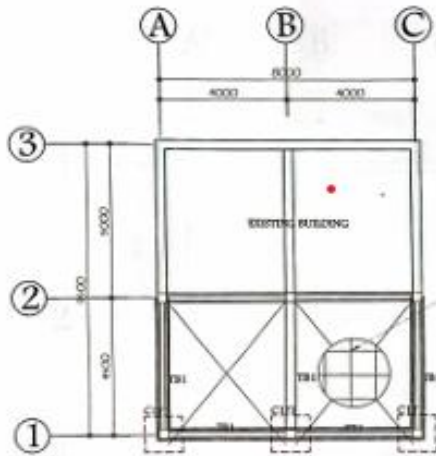
FOUNDATION PLAN SCALE 1:500
